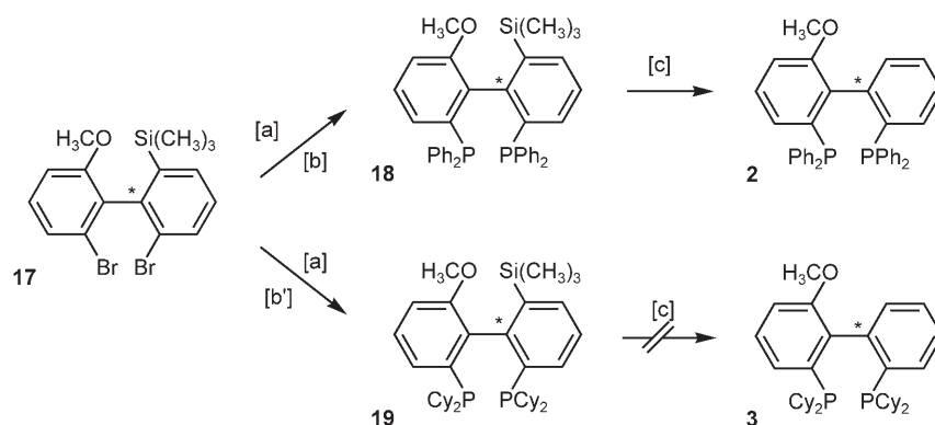
Scheme 6. Attempt to use silylated precursors. Reagents and conditions: [a] Butyllithium (2.0 equivs.) in toluene at -75^{\circ}\text{C} . [b] Chlorodiphenylphosphine (2.0 equivs.). [b'] Chlorodicyclohexylphosphine (2.0 equivs.). [c] TBAF·H 2 O in DMF at 120^{\circ}\text{C} , 3 days.
