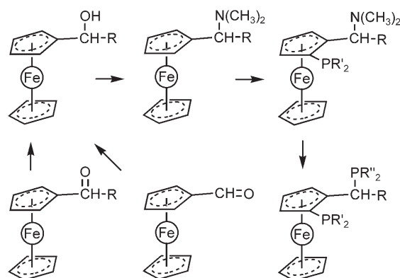
Scheme 1. Modular synthetic access to ferrocene based ligands.
