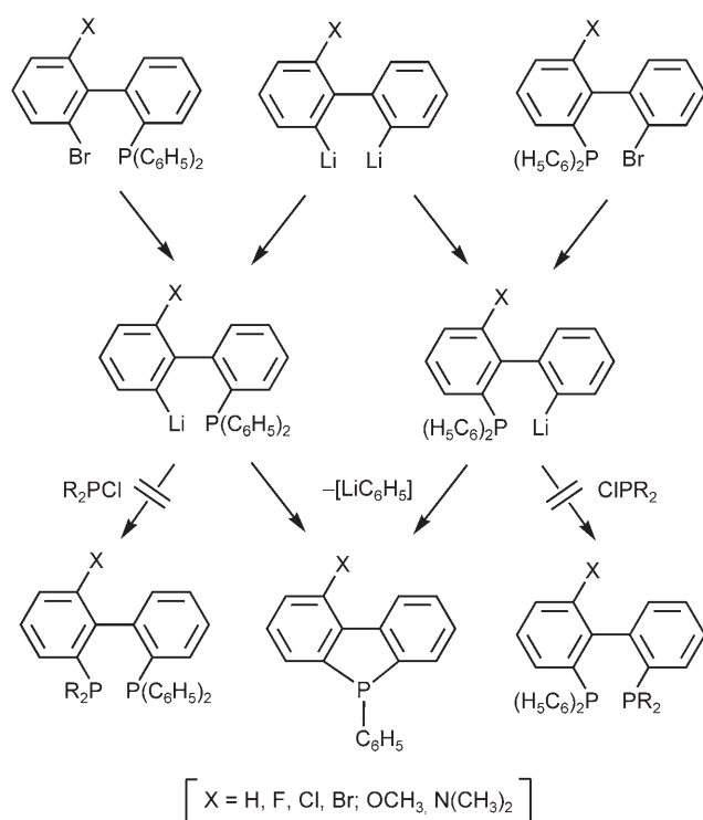
Scheme 3. Formation of “9-phosphafluorenes”.
