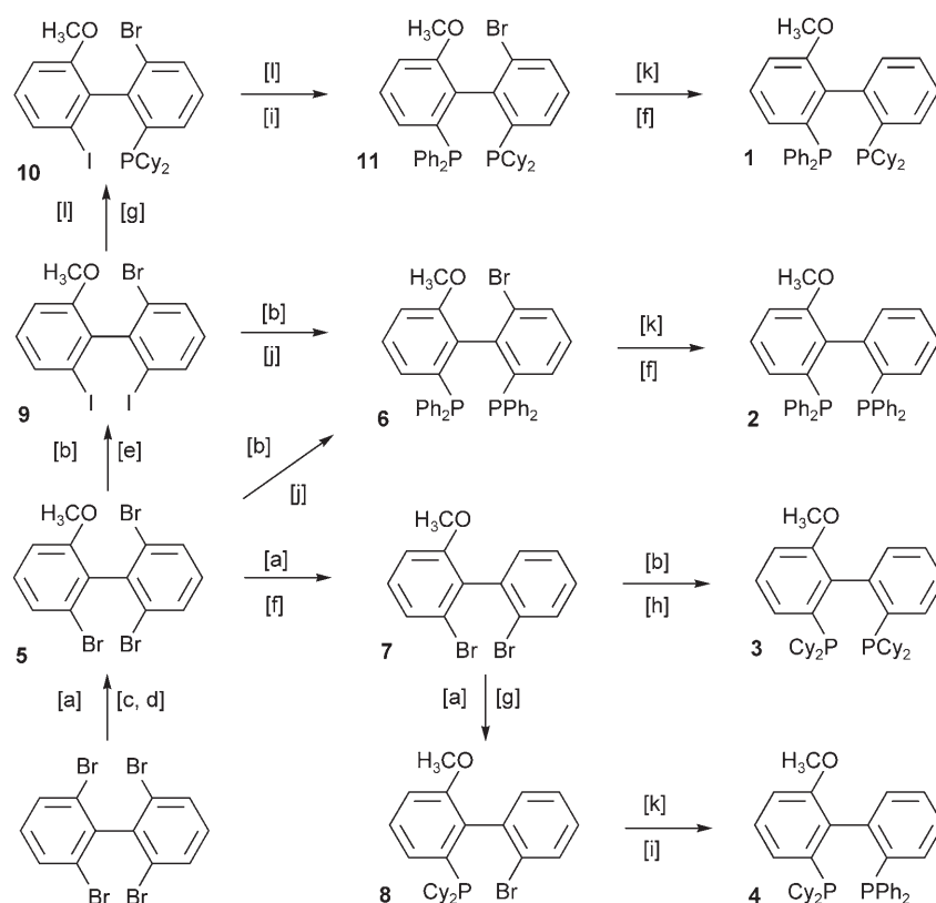
Scheme 4. Modular synthetic access to atropisomeric biphenyl ligands. Reagents and conditions: [a] Butyllithium (1.0 equiv.) in tetrahydrofuran (THF) at -75^{\circ}\text{C} . [b] Butyllithium (2.0 equivs.) in THF at -75^{\circ}\text{C} . [c] (i) Fluorodimethoxyborane-diethyl etherate; (ii) aqueous sodium hydroxide/hydrogen peroxide. [d] Methyl iodide, potassium hydroxide in dimethyl sulfoxide. [e] Iodine (2.0 equivs.). [f] Methanol. [g] Chlorodicyclohexylphosphine (1 equiv.). [h] Chlorodicyclohexylphosphine (2.0 equivs.). [i] Chlorodiphenylphosphine (1.0 equiv.). [j] Chlorodiphenylphosphine (2.0 equivs.). [k] Butyllithium (2.0 equivs.) in toluene at +25^{\circ}\text{C} . [l] Butyllithium (1.0 equiv.) in diethyl ether (DEE) at -75^{\circ}\text{C} .
