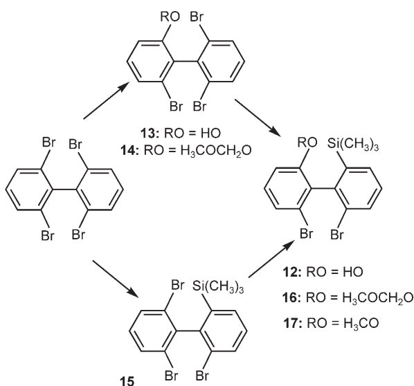
Scheme 5. Racemate resolution of a common precursor.
