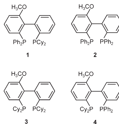
Scheme 2. Four target ligands demonstrating the modular construction of biaryl-based ligands.
